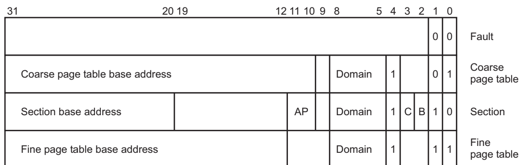
Figure 7-4 Level one descriptor
